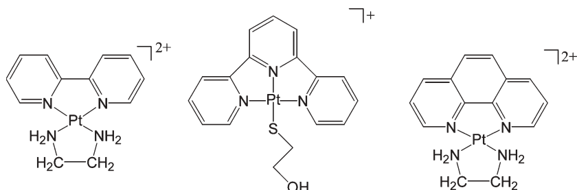
Fig. 12 Platinum complexes [\text{Pt}(\text{bipy})(\text{en})]^{2+} , [\text{Pt}(\text{terpy})(\text{HET})]^+ and [\text{Pt}(\text{o-phen})(\text{en})]^{2+} . 12
