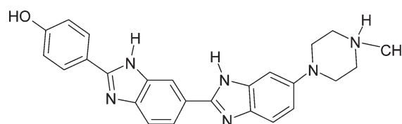
Fig. 4 Chemical structure of a typical minor groove binder Hoechst 33258.
