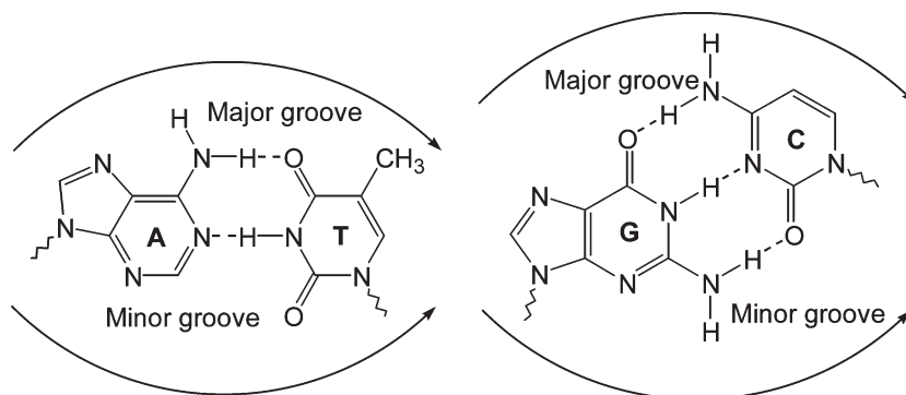
Fig. 3 Adenine–thymine and guanine–cytosine base pairs showing the minor and major grooves. The wiggly bonds indicate the links to the sugar backbone.
